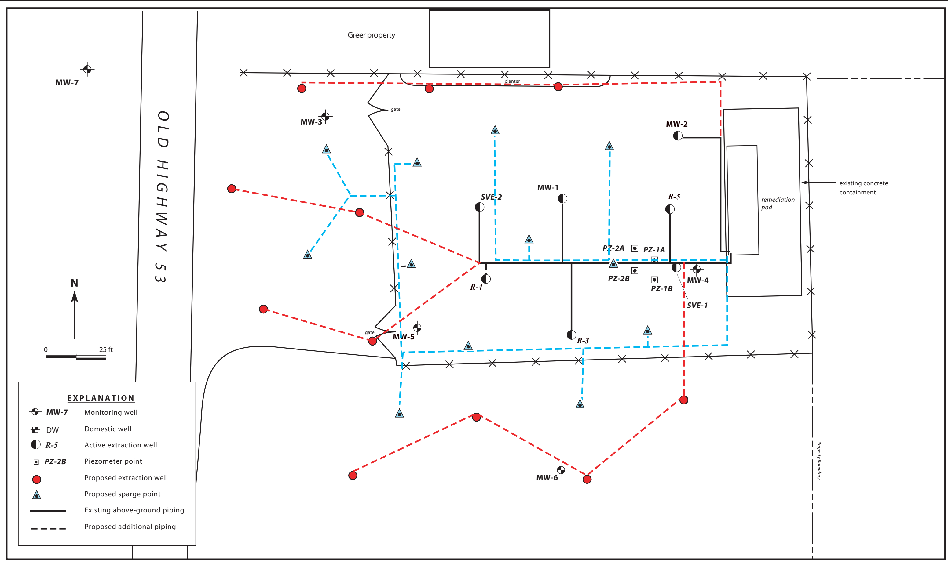
Figure 2. Proposed Remediation System Expansion - Phase 2 - Former Chevron Bulk Plant, 5200 Old Highway 53, Clearlake, California
