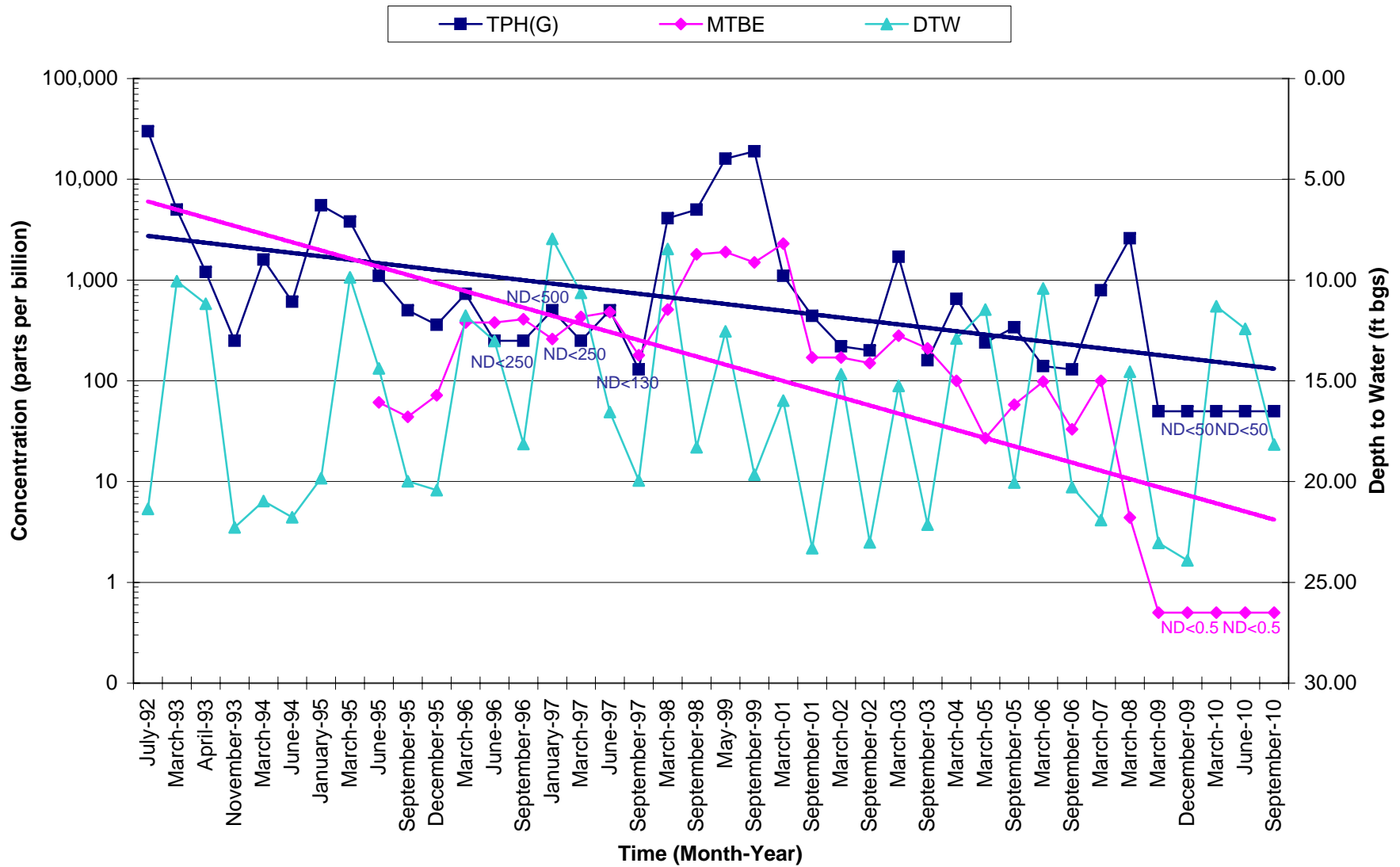
Graph 3: Gasoline and MTBE Concentrations and Depth to Water versus Time in Well MW-3 - Gavilan College - 5055 Santa Teresa Boulevard, Gilroy, California
